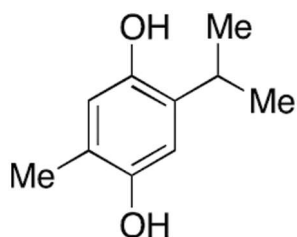
thymohydroquinone
