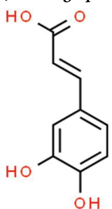
caffeic acid
