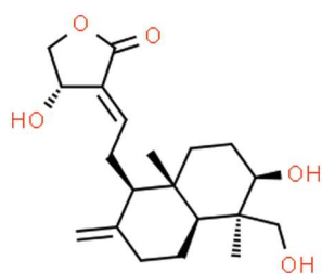
isoandrographolide
