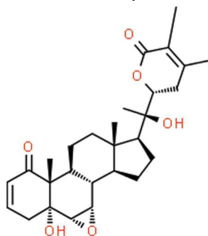
Withanol
