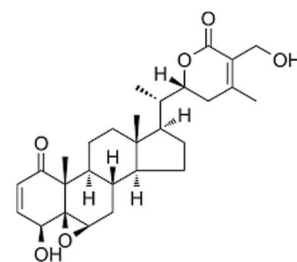
withaferine A
