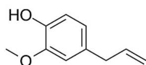
Eugenol
