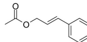
cinnamyl acetate
