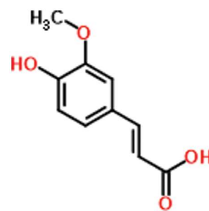
ferulic acid
