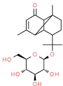
Tinocordiside
