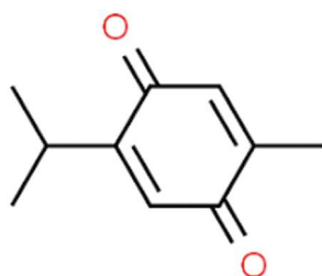
Thymoquinone
